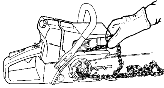
Place chain onto the sprocket
