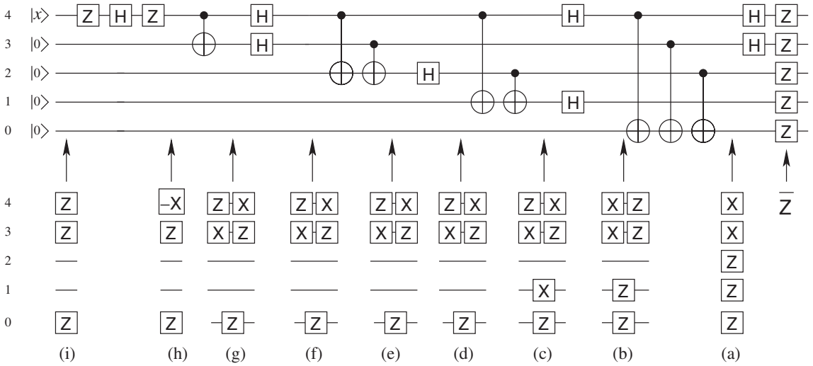
Fig 5.18 Demonstration that \bar{Z} = Z_0Z_1Z_2Z_3Z_4 acting on the output of the encoding circuit in Figure 5.11 is the same as Z_4Z_3Z_0 acting on the input, which takes |x0000\rangle into (-1)^x|x0000\rangle .
