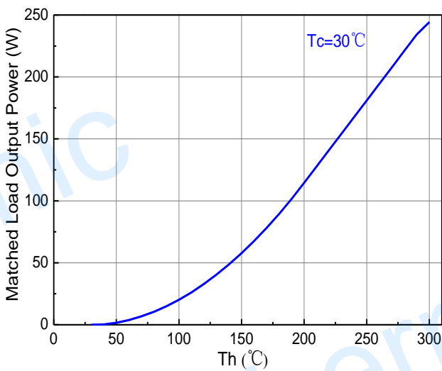
The chart for matched load output power Vs Th under Tc=30°C input water temperature
