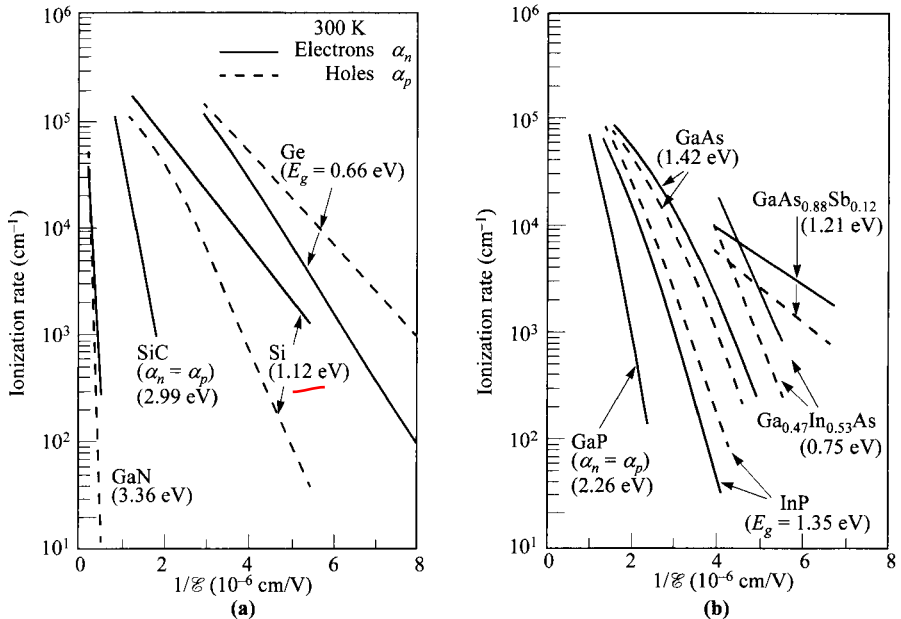
Fig. 23 Ionization rates at 300 K versus reciprocal electric field for Si, GaAs, and some IV-IV and III-V compound semiconductors. (After Refs. 55–65.)
