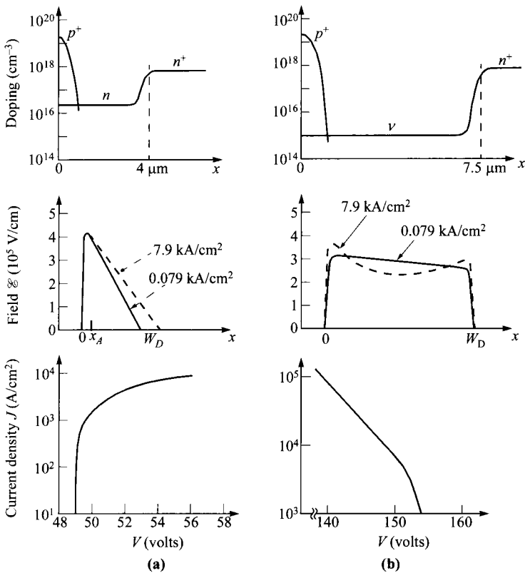
Fig. 4 Doping profile, field, and current-voltage characteristics of (a) p^+ - n - n^+ and (b) p^+ - v - n^+ diodes. Area = 10^{-4} \text{ cm}^2 . (After Ref. 14.)
