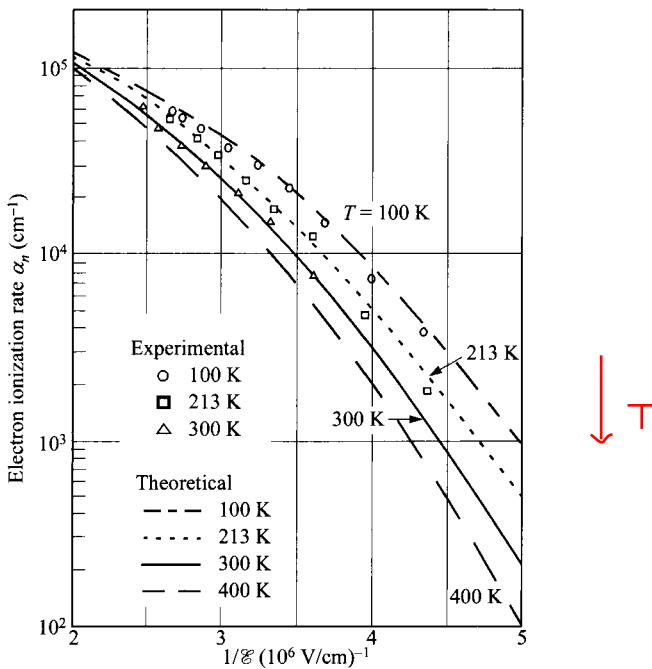
Fig. 24 Electron ionization rate versus reciprocal electric field in Si for four temperatures. (After Ref. 66.)
