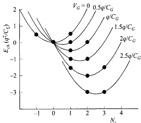
Fig. 56 E_{ch} vs. N_i for different V_G to determine N_i in single-electron box. It can be seen that depending on V_G , the E_{ch} minimum falls on either single or double values of N_i .
