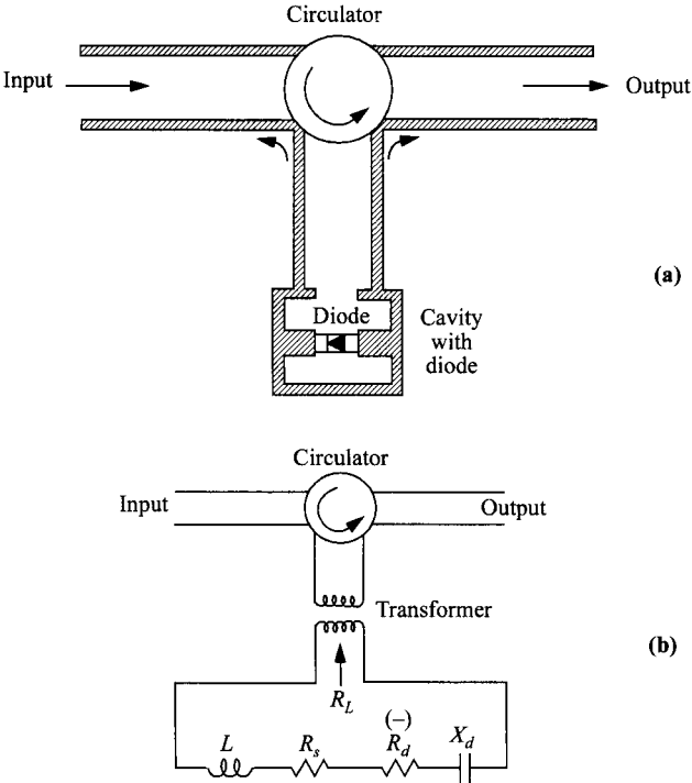
Fig. 13 (a) IMPATT diode inserted into a resonator. (b) Equivalent circuit. (After Ref. 30.)
