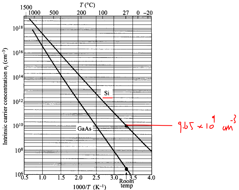
Fig. 9 Intrinsic carrier concentrations of Si and GaAs as a function of reciprocal temperature. (After Refs. 22 and 29.)
