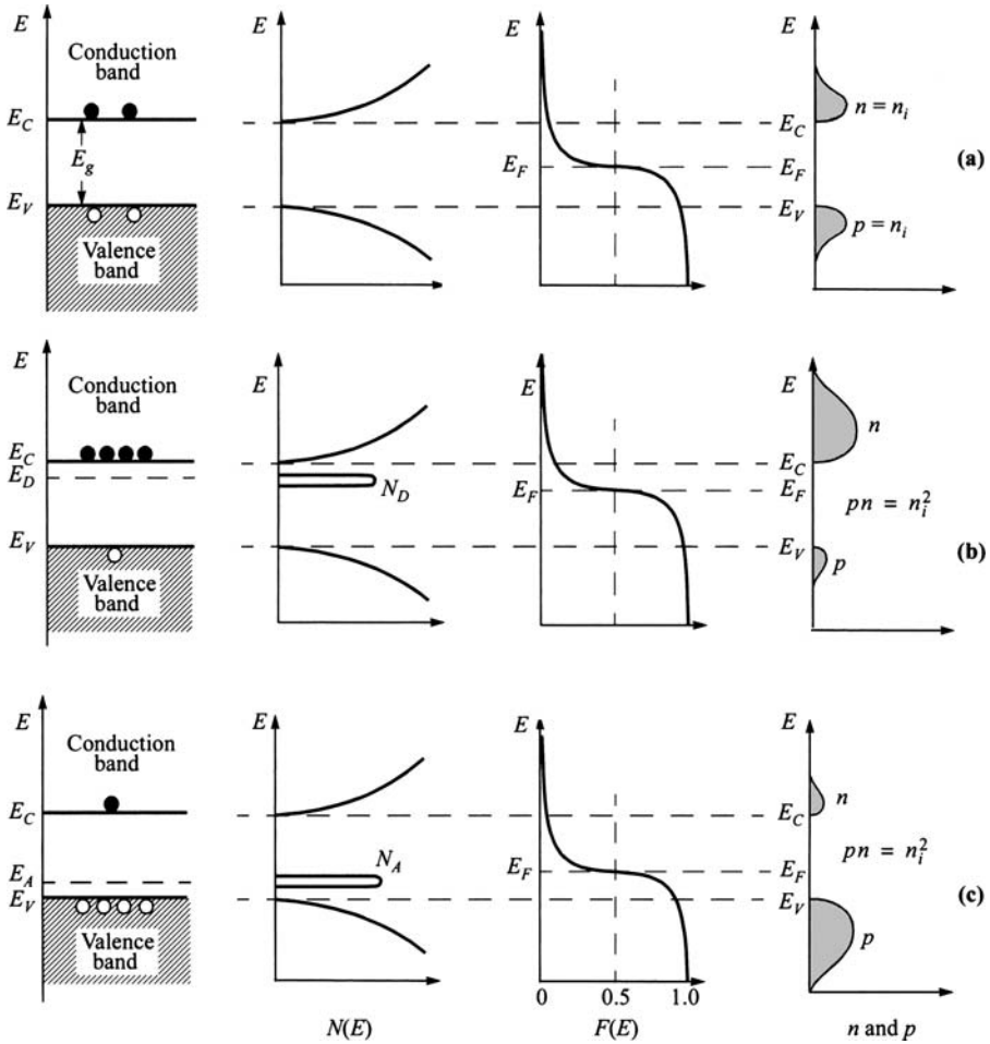
Fig. 11 Schematic band diagram , density of states , Fermi-Dirac distribution , and carrier concentrations for (a) intrinsic, (b) n -type, and (c) p -type semiconductors at thermal equilibrium . Note that pn = n_i^2 for all three cases.
