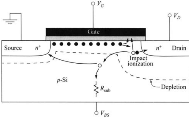
Fig. 30 Current components of a MOSFET under high fields.
