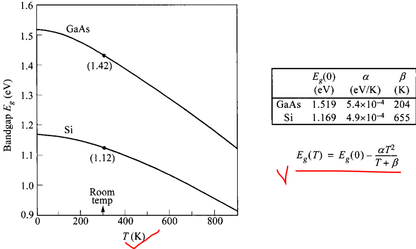
Fig. 6 Energy bandgaps of Si and GaAs as a function of temperature. (After Refs. 22–23.)
