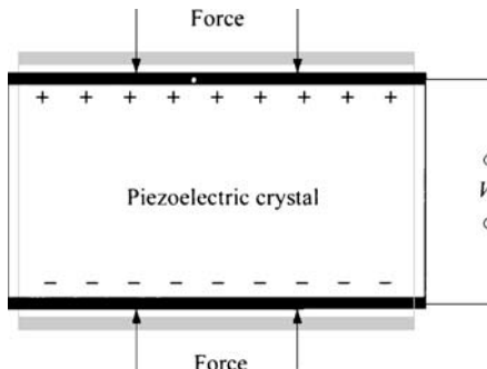
Fig. 7 In a piezoelectric transducer, strain produces charge (and voltage), and vice versa.
