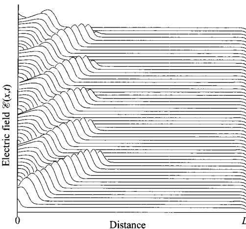
Fig. 12 Numerical simulation of TED in quenched dipole-layer mode. (After Ref. 28.)
